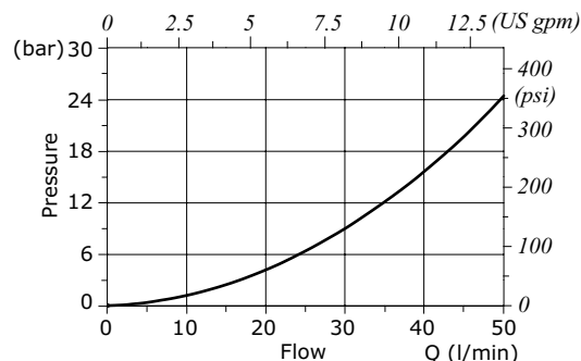
RP10W pressure drop vs. flow 2-&gt;1
