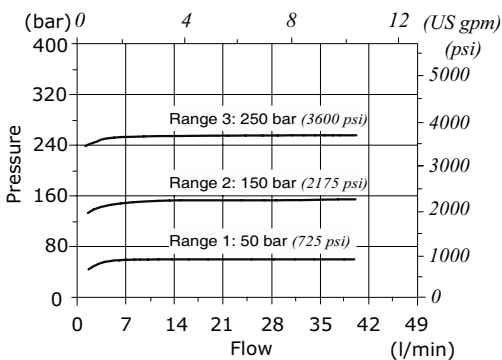
MC10A pressure vs. flow Std. setting at 5 l/min (1.32 US gpm)
