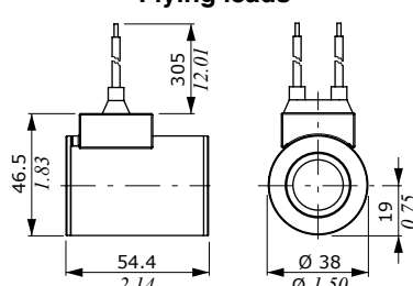
Flying leads
