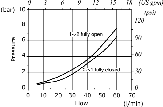
NT12A pressure drop vs flow
