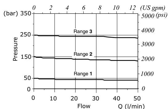
RM10A pressure reducing vs. flow 2-&gt;1
