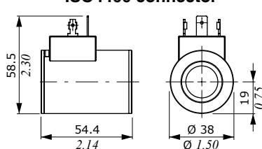
ISO4400 connector
