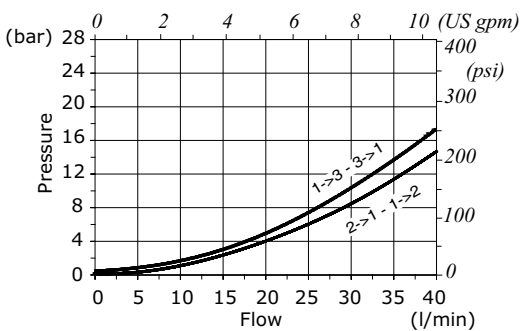
EJ10M pressure drop vs. flow - Spool 5 -
