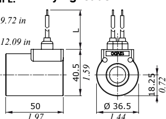
Flying leads with DEUTSCH DT04 connector
