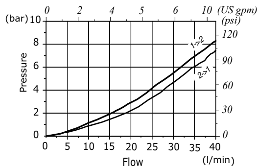
EC08M/10NB - EC08M/20NB pressure drop vs. flow
