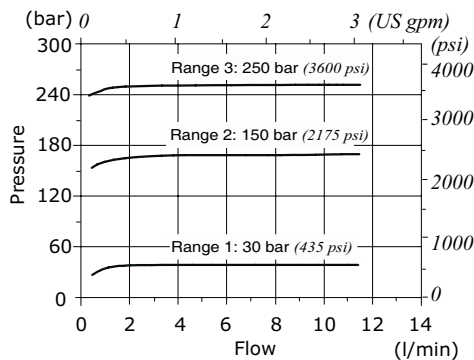
MC08A pressure vs. flow Std. setting at 5 l/min (1.32 US gpm)
