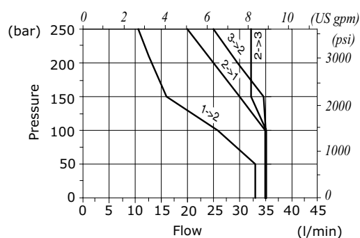
EJ10M performance limit
