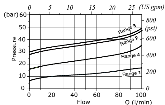
RP12W pressure drop vs. flow 1-&gt;3 with de-energized coil
