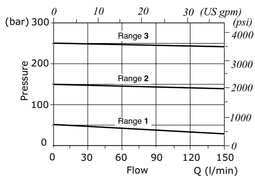
RM16A pressure reducing vs. flow 2-&gt;1
