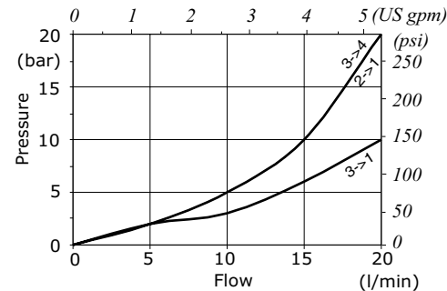
ER08M pressure drop vs. flow - Spool 8 -
