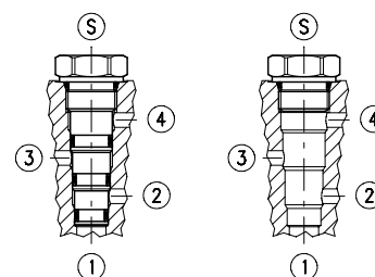
Cavity plugs
