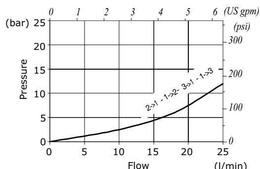
EJ10Mp pressure drop vs. flow
