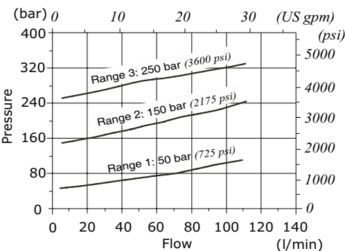
MC12A pressure vs. flow Std. setting at 5 l/min (1.32 US gpm)
