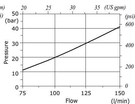
PD16C pressure drop vs flow from 2->1/3 and from 1/3->2
