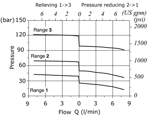
RD08A reducing/relieving pressure vs. flow
