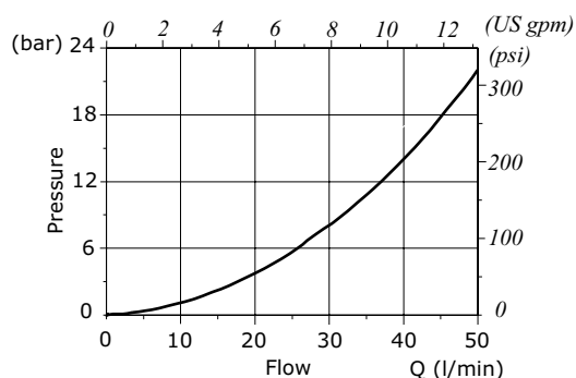
RM10A pressure drop vs. flow 2-&gt;1
