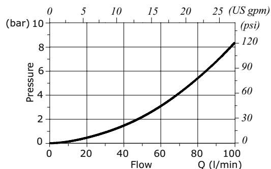
RP12W pressure drop vs. flow 2-&gt;1
