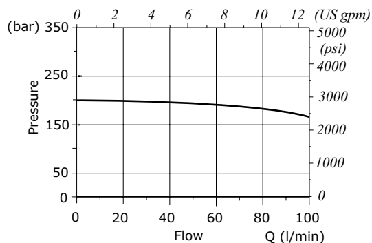
RM12A pressure reducing vs. flow 2-&gt;1
