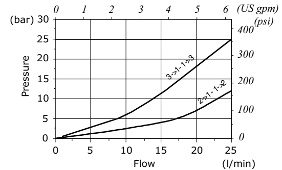
EJ08M pressure drop vs. flow
