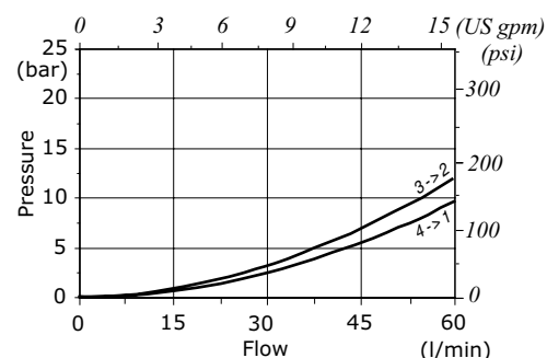
ER12M pressure drop vs. flow - Spool 2 -
