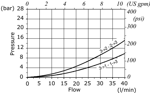
EJ10M pressure drop vs. flow - Spool 6 -
