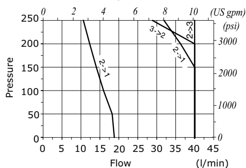
EJ10M performance limit
