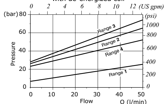
RP10W pressure drop vs. flow 1-&gt;3 with de-energized coil
