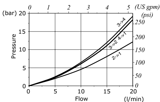
ET08M pressure drop vs. flow - Spool 4 -
