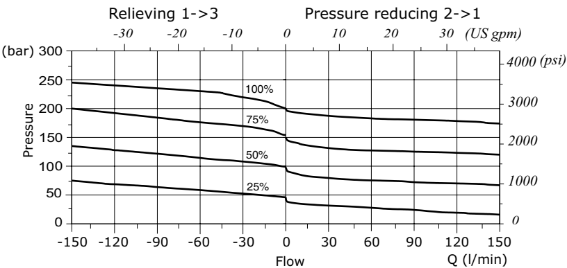
RP16W reducing/relieving pressure vs. flow for % of control current - Pressure range 2 -
