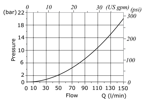
RM16A pressure drop vs. flow 2-&gt;1
