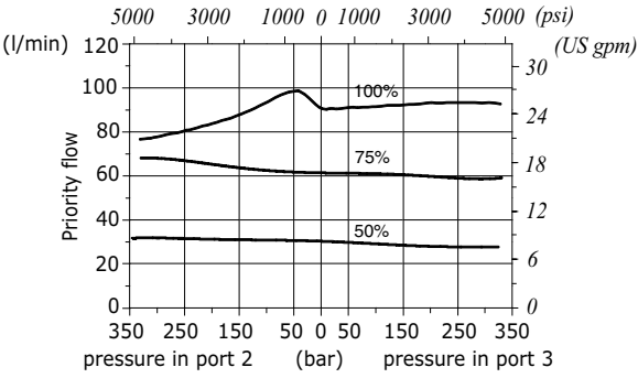
PP16X pressure compensation diagram 2→3 for % of control current - with Q1=100 l/min
